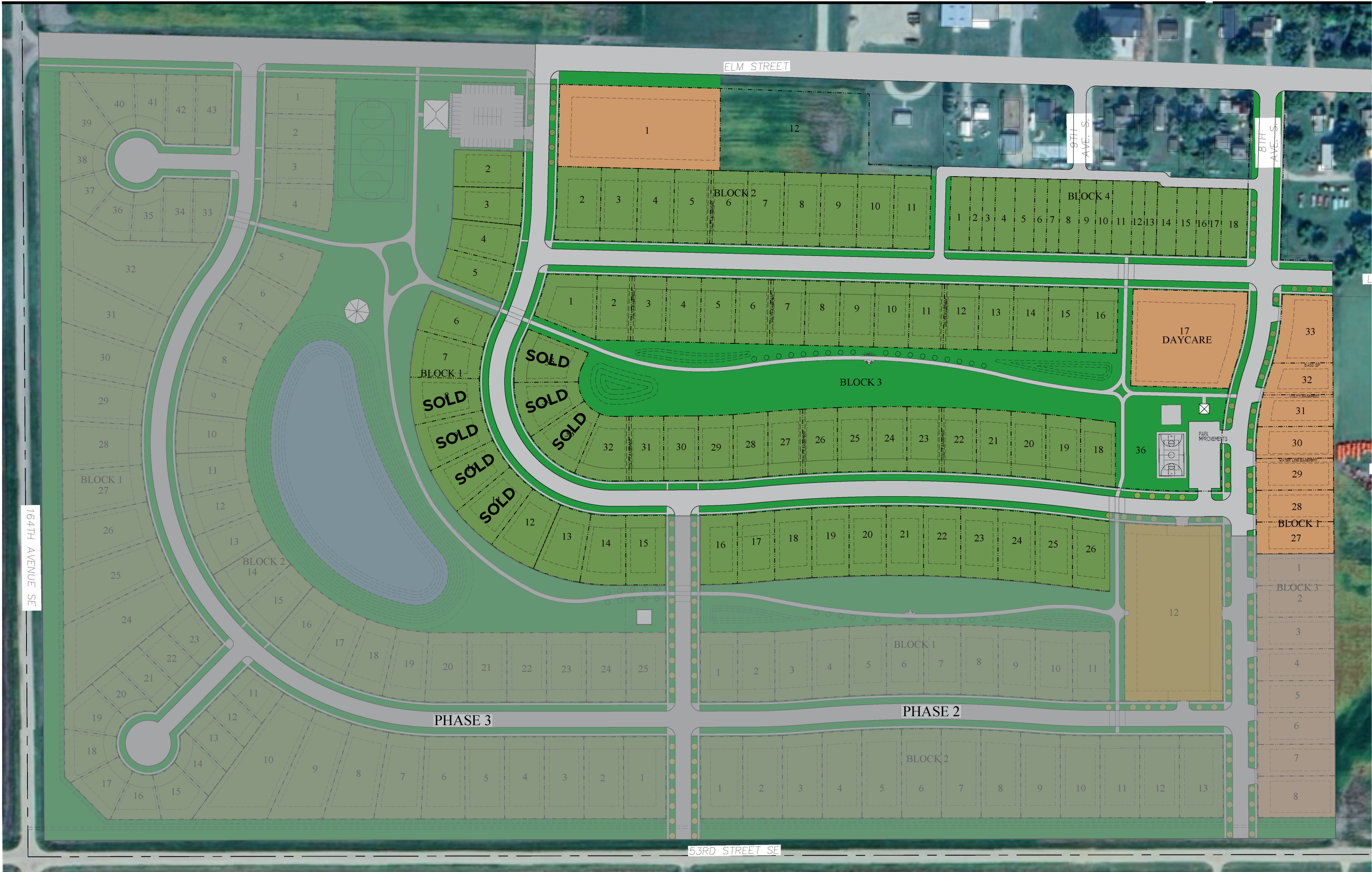
1 SITE PLAN 1" = 80'-0"
